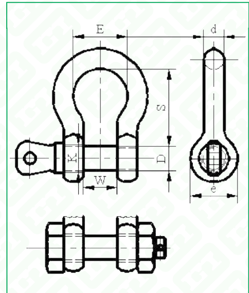
(GM 209) Anchor Shackle With Screw Pin &amp; (GM 2130) Anchor Shackle With Bolt Pin
