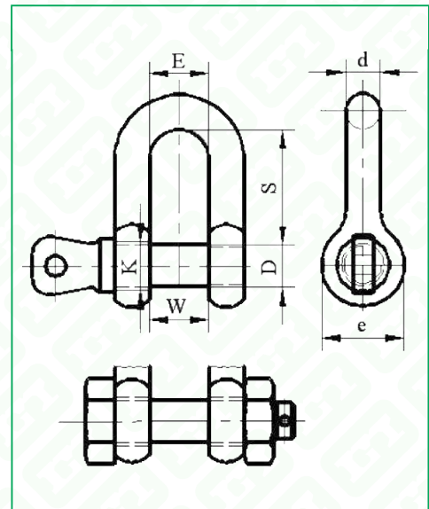
(GM 210) Chain Shackle With Screw Pin &amp; (GM 2150) Chain Shackle With Bolt Pin
