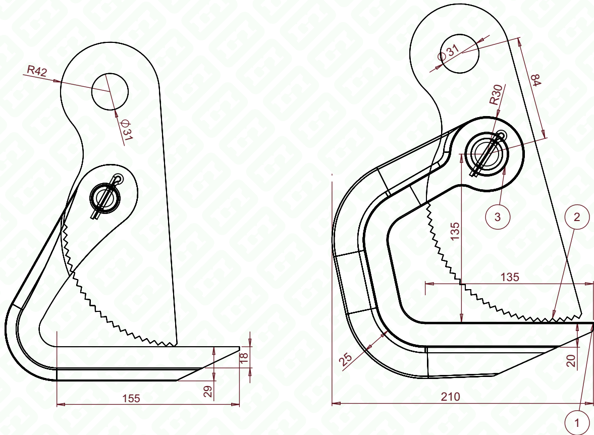
2.5 TONS 0-60 mm
